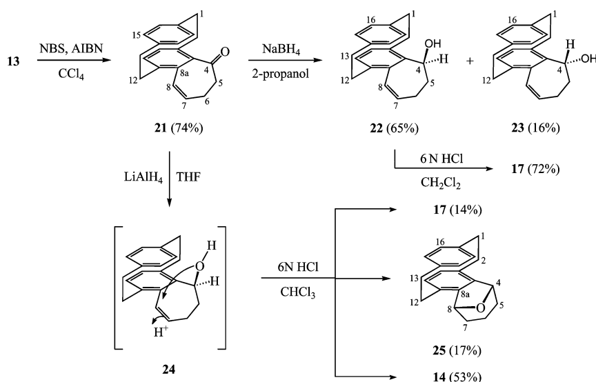
Scheme 5. Some reactions of annulated [2.2]paracyclophanes.
