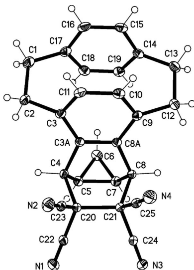
Figure 6. The molecule of compound 28 in the crystal. Ellipsoids represent 30% probability levels.
