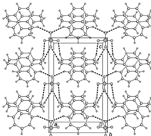
Figure 8. Packing diagram for compound 26b viewed parallel to the y axis. C–H \cdots O interactions are indicated by thick dashed bonds.
