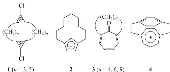
Scheme 1. A selection of nonbenzenoid cyclophanes.
