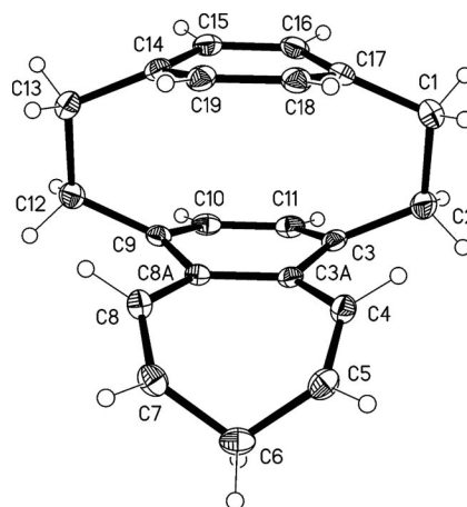
Figure 2. The molecule of compound 17 in the crystal. Ellipsoids represent 30% probability levels.
