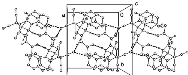
Figure 10. Packing diagram for compound 29 viewed parallel to the z axis. C–H \cdots O interactions are indicated by thick dashed bonds. H atoms not involved in short contacts are omitted for clarity.
