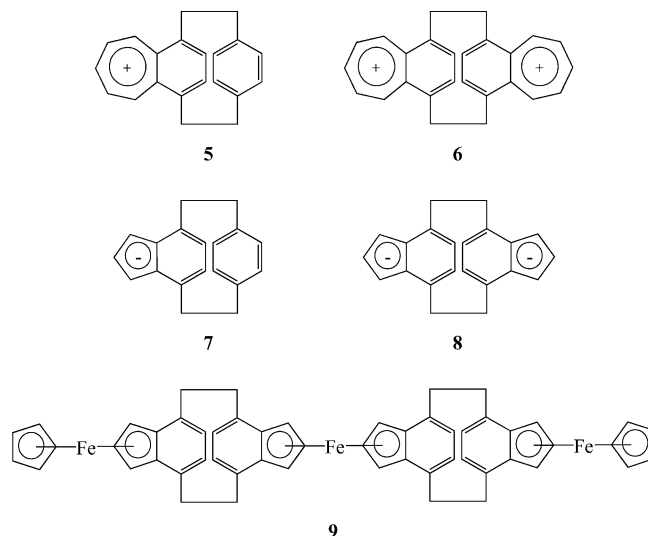
Scheme 2. Charged [2.2]phanes with 10 \pi -electron decks.
