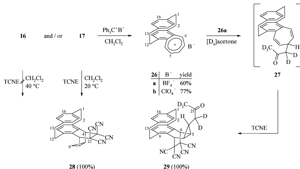
Scheme 6. Preparation of tropyliophanes 26 .
