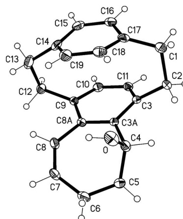
Figure 3. The molecule of compound 22 in the crystal. Ellipsoids represent 30% probability levels.
