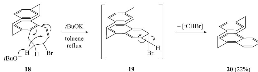
Scheme 4. Fragmentation of 18 to naphthalenophane 20 .
