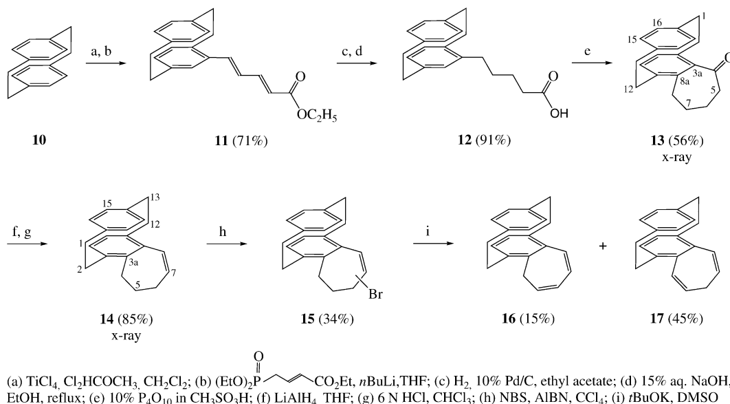
Scheme 3. Annulation of a seven-membered ring to [2.2]paracyclophane ( 10 ).
