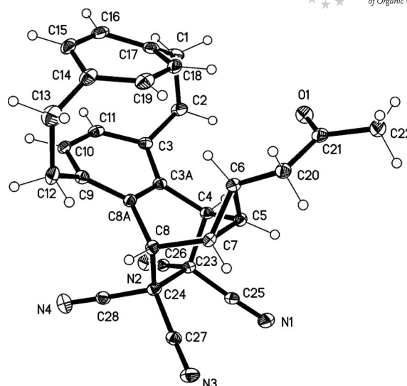
Figure 7. The molecule of compound 29 in the crystal (excluding the solvent molecule). Ellipsoids represent 30% probability levels.
