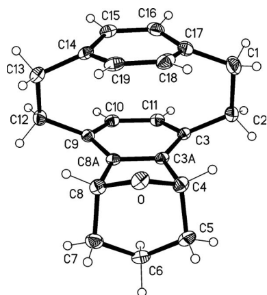
Figure 4. The molecule of compound 25 in the crystal. Ellipsoids represent 30% probability levels.
