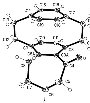
Figure 1. The molecule of compound 13 in the crystal. Ellipsoids represent 30% probability levels.
