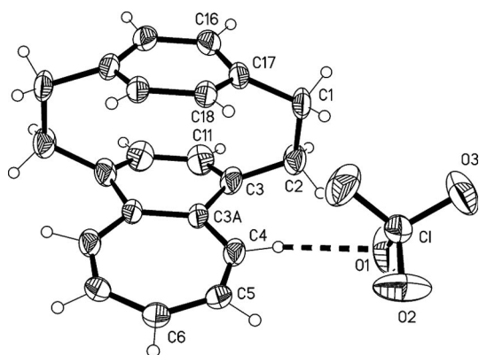
Figure 5. The formula unit of compound 26b in the crystal. Only the asymmetric unit is numbered. Ellipsoids represent 30% probability levels.
