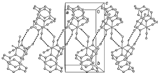
Figure 9. Packing diagram for compound 28 viewed parallel to the z axis. C–H \cdots O interactions are indicated by thick dashed bonds. H atoms not involved in short contacts are omitted for clarity.
